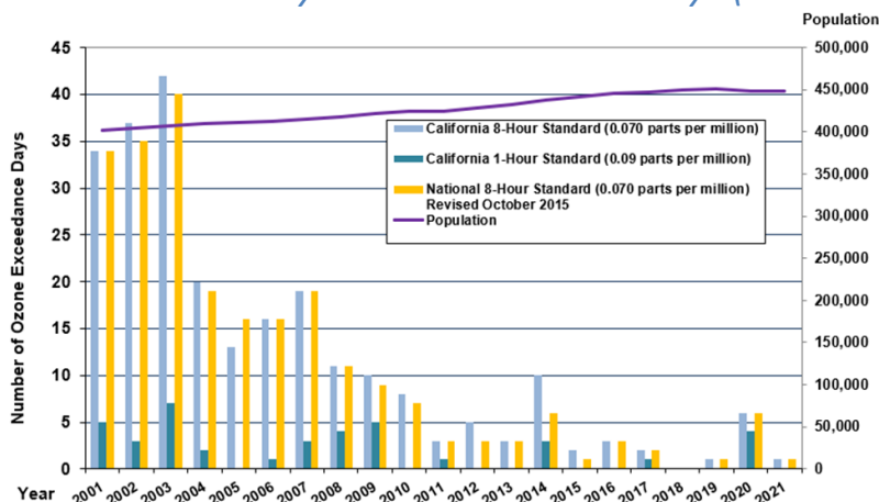
Santa Barbara County Ozone Exceedance Days (2001-2021)
