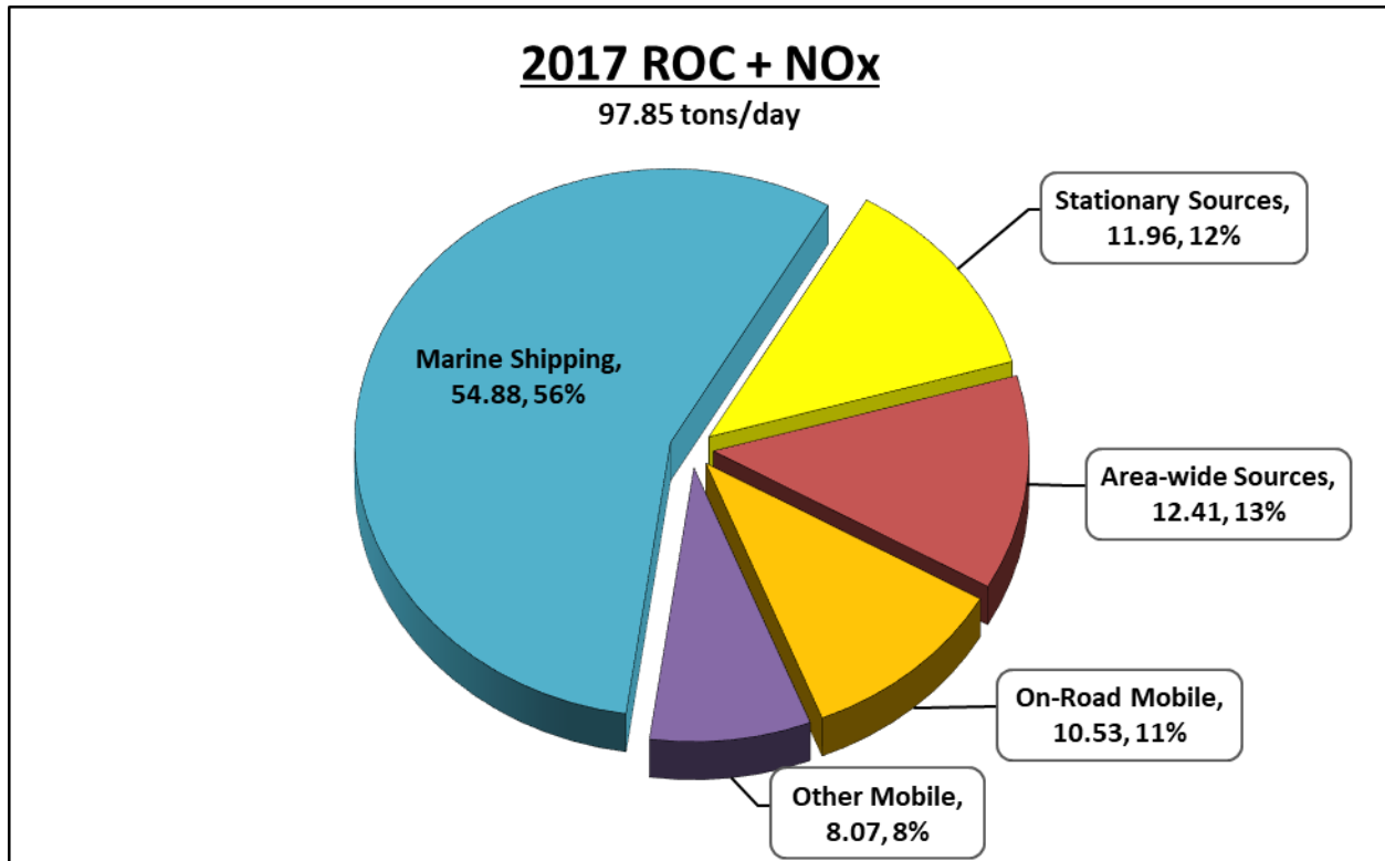
FIGURE 3-2: COMBINED BASELINE ROC AND NO x EMISSIONS (TONS PER DAY) AND DISTRIBUTION (%)
