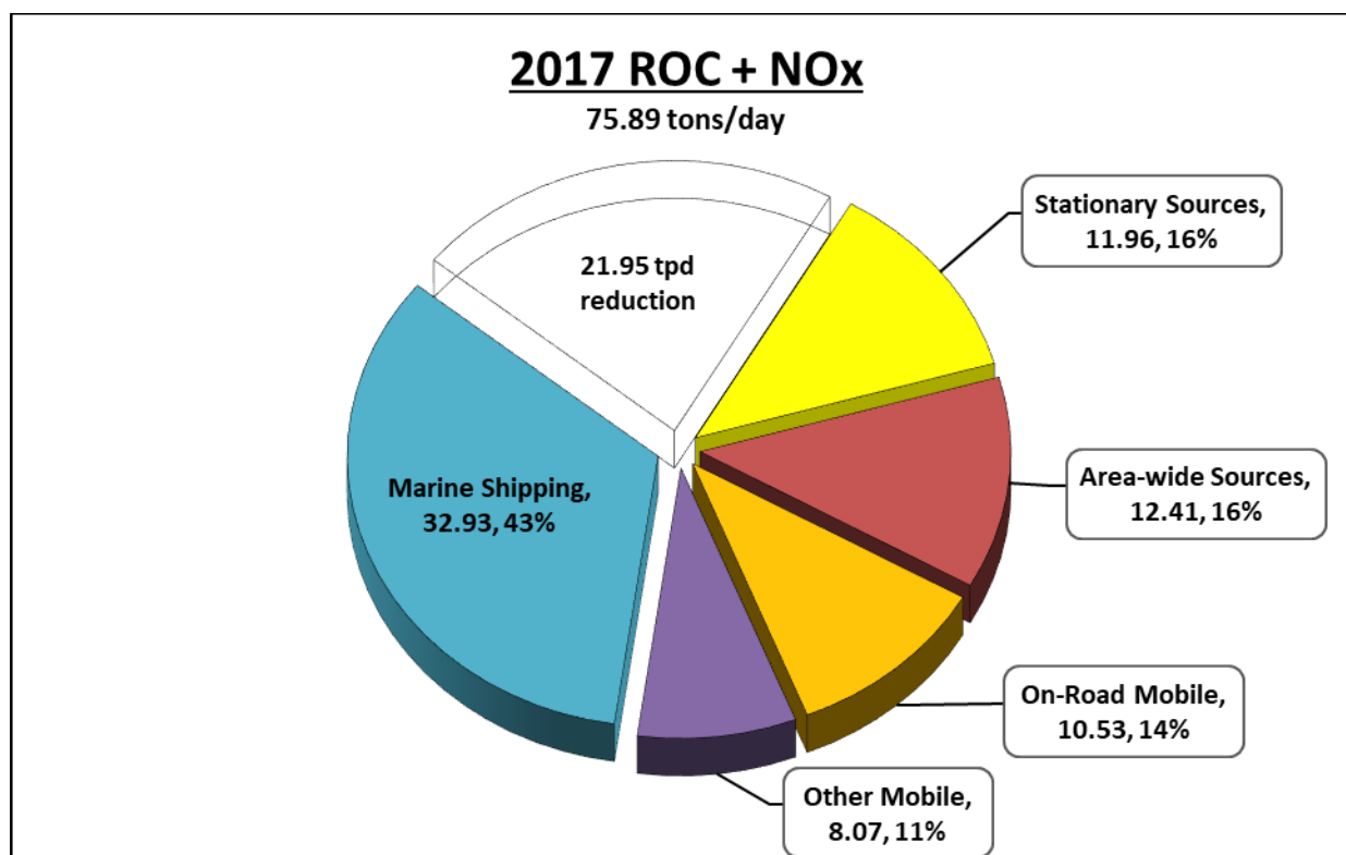
FIGURE 3-4: REDUCED MARINE SHIPPING METHODOLOGY - COMBINED BASELINE ROC AND NOx EMISSIONS (TONS PER DAY) AND DISTRIBUTION (%)
