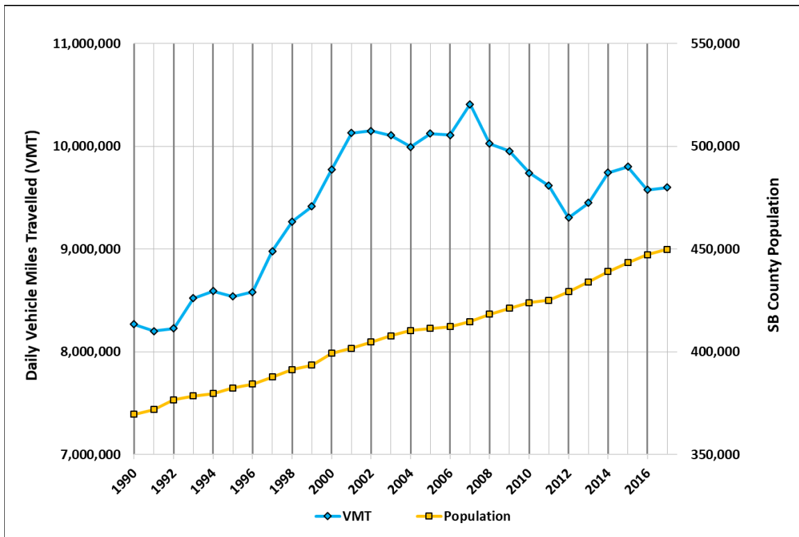
FIGURE 5-1: POPULATION AND DAILY VMT TRENDS SANTA BARBARA COUNTY, 1990-2017 18
