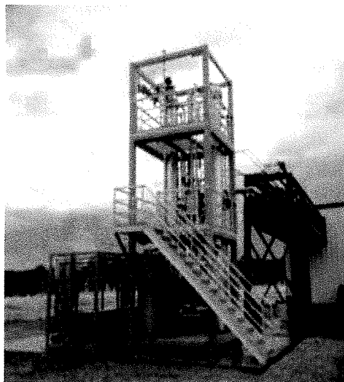
Distillation & dehydration modules installed at the University of Florida Stan Mayfield Biofuel Center
